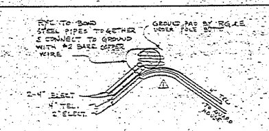
PLAN OF NEW POLE NO SCALE
